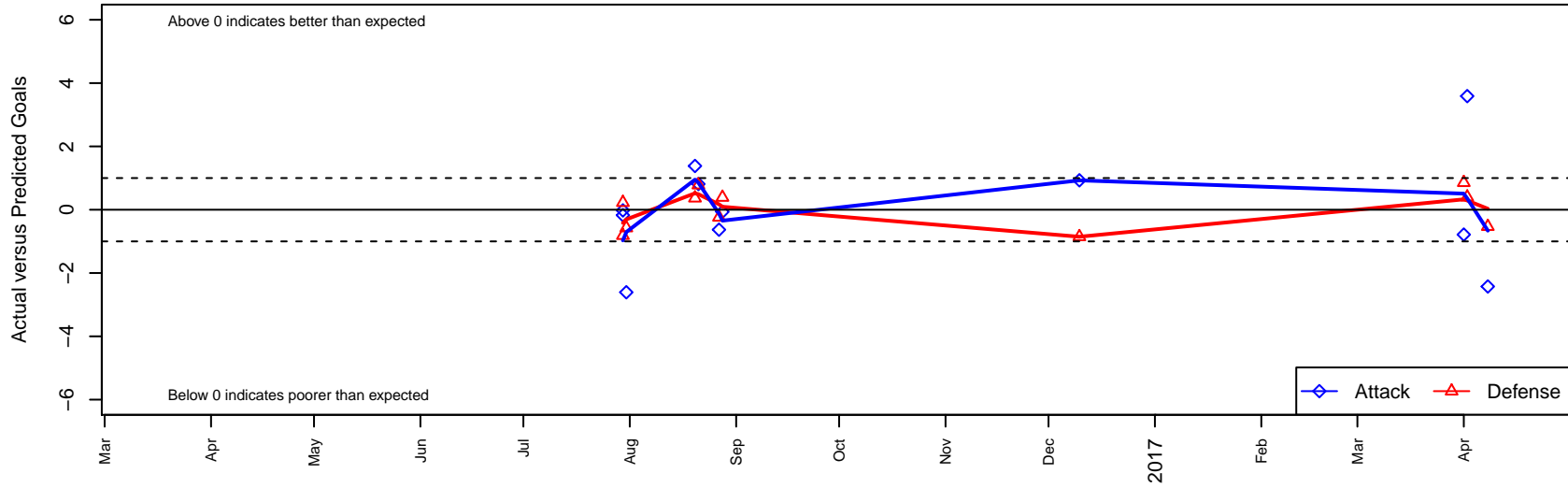
Legends FC South G00 Dots are actual minus expected GF (blue circles) and GA (red triangles). Blue line is smoothed change in attack strength. Red is smoothed change in defense strength.
